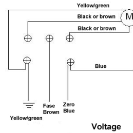
Connection diagram Presto and Geba switch
