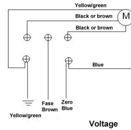
Connection diagram Presto and Geba switch
